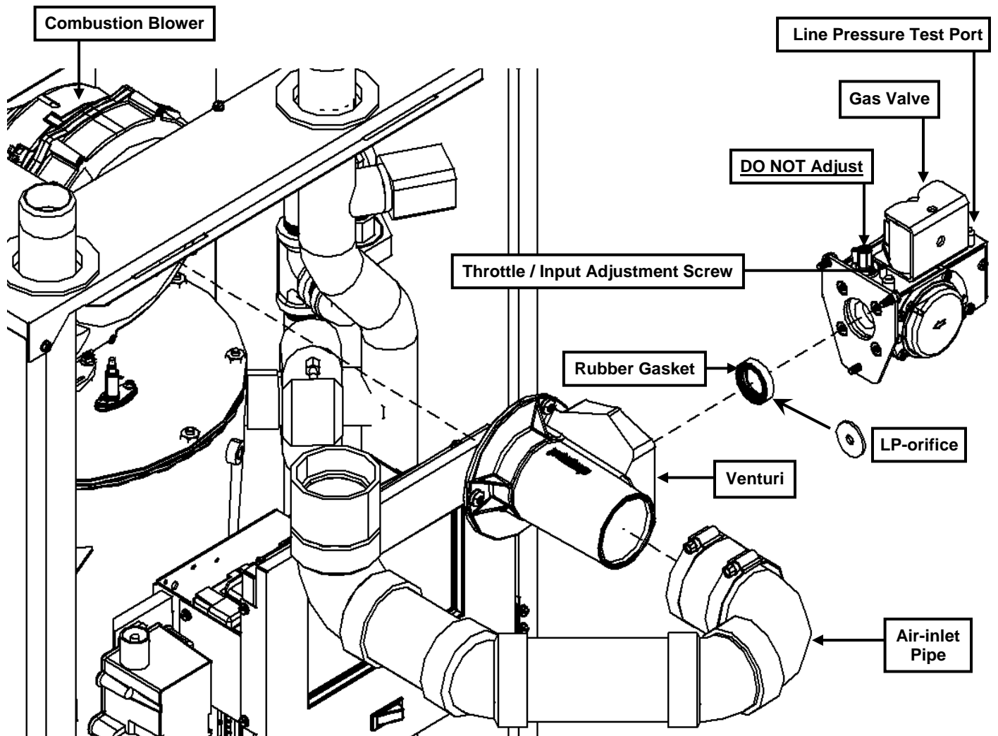
Figure 1-1 LP-Orifice and Throttle/Input Screw Adjustment
