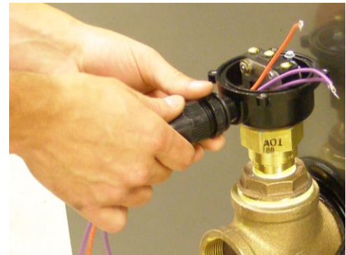
Fig. 5 - Flow Switch Wiring
