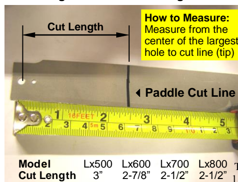
Fig. 2 - Paddle Cut Lengths
